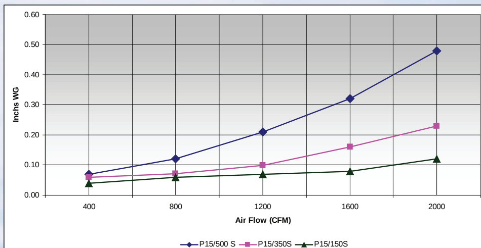
Pressure Drop - Resistance Curve
